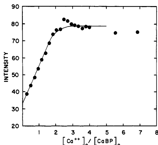
FIGURE 6: \text{Ca}^{2+} titration data. The resonance intensity (in arbitrary units) at 7.16 ppm in Figure 5 is plotted vs. the ratio of total \text{Ca}^{2+} concentration to total ICaBP concentration. The protein was found to initially be 14% saturated with calcium after desalting (see the text).
